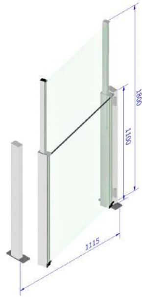
Wind Barrier with steel base
